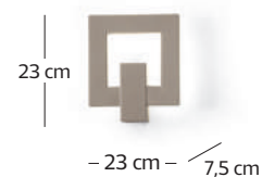
art. Ri_quadro A20 LED 1260 LM 12 W 3000 K
