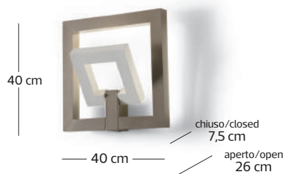
art. Ri_quadro A40-2 LED 3510 LM 32 W 3000 K
